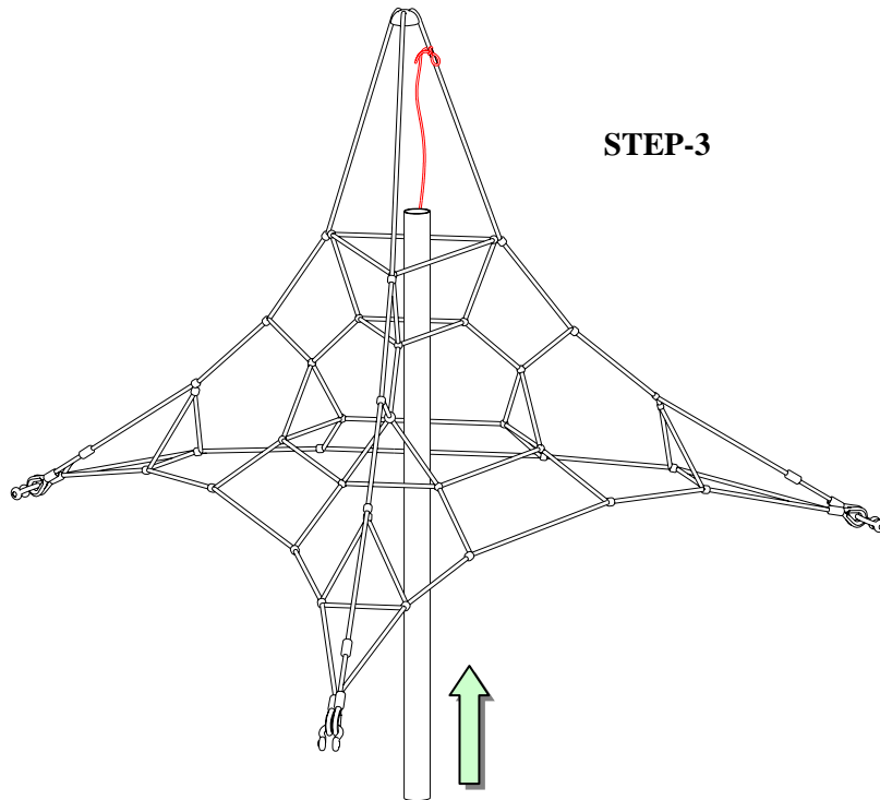
Figure-13: Insert Post into the Center of Net.
