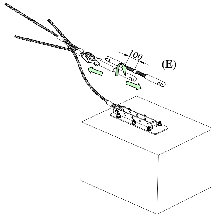
Figure-20: Loosen Turnbuckle: all the way (about 100mm), leaving only 4 or 5 threads attached
