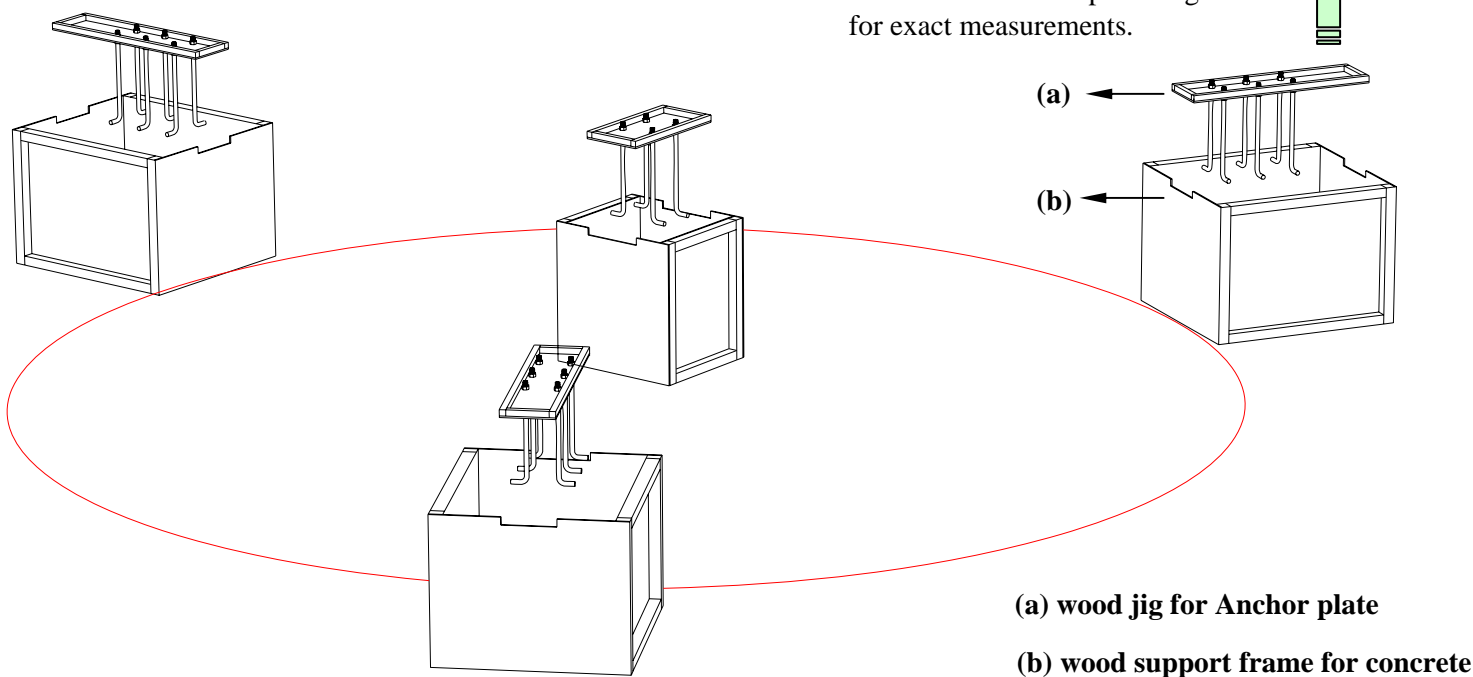
Figure-6: Wood support frame
