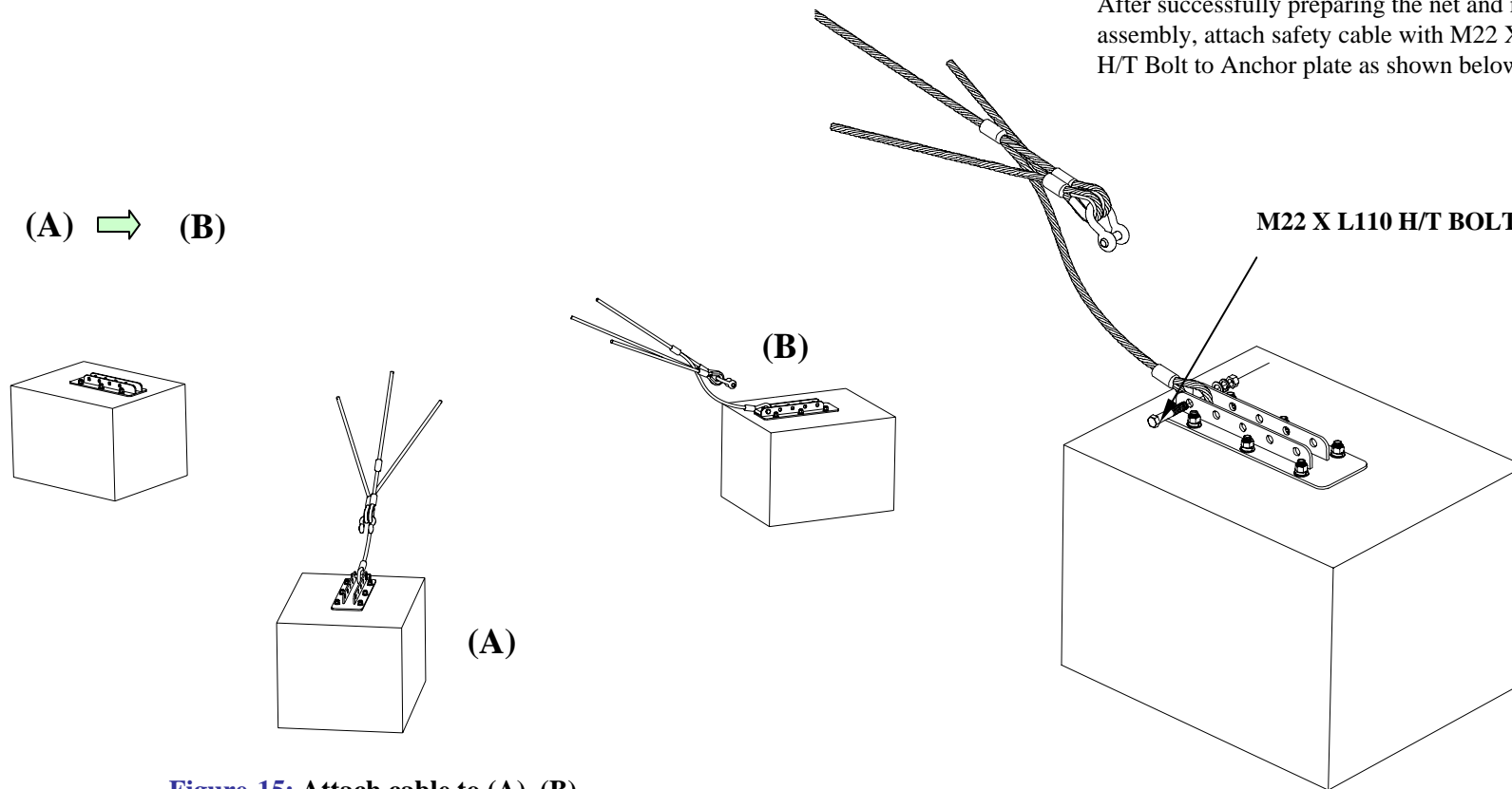
Figure-15: Attach cable to (A) (B)
