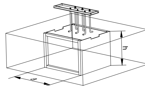
Figure-3: Excavate enough materials to allow for proper depth of concrete footings
